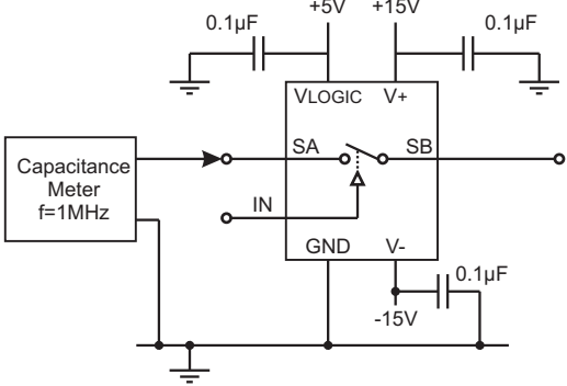
Figure 8 - Off Capacitance
