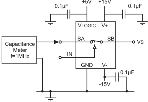
Figure 9 - On Capacitance
