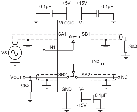
Figure 7 - Channel-to-Channel Crosstalk
