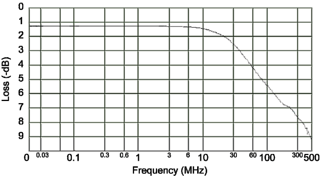
Figure 10. Frequency Response.
