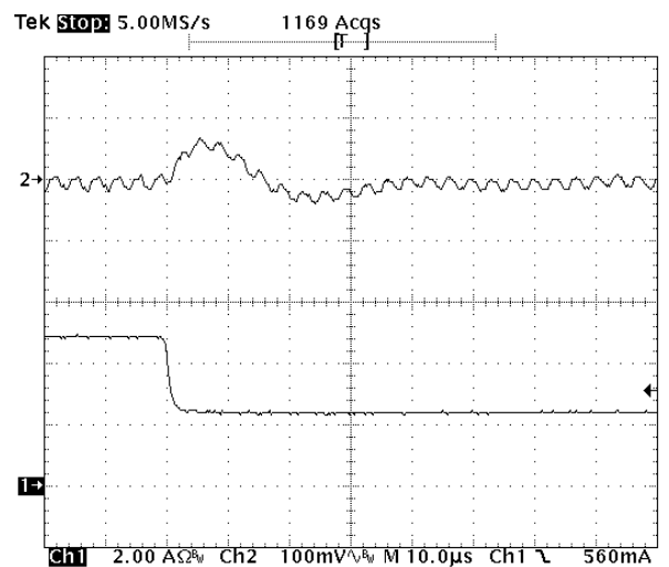
Fig-2.0V-7: Output voltage response for V_{out}=2.0V to positive load current step-change from 5A to 2.5A with slew rate of -5A/\mu s at V_{in}=5.0V . C_o=47\mu F \times 2 ceramic.
