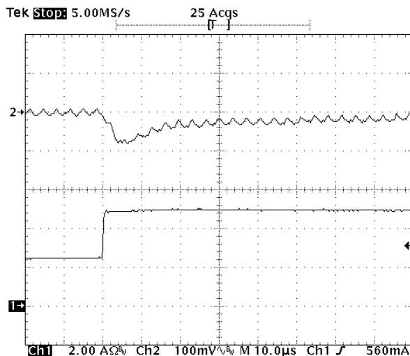
Fig-3.3V-6: Output voltage response for V_{out}=3.3V to positive load current step-change from 2.5A to 5A with slew rate of 5A/\mu s at V_{in}=5.0V . C_o=47\mu F \times 2 ceramic.
