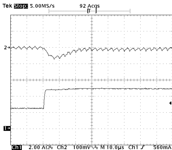
Fig-1.0V-6: Output voltage response for V_{out}=1.0V to positive load current step-change from 2.5A to 5A with slew rate of 5A/\mu s at V_{in}=5.0V . C_o=47\mu F \times 2 ceramic.
