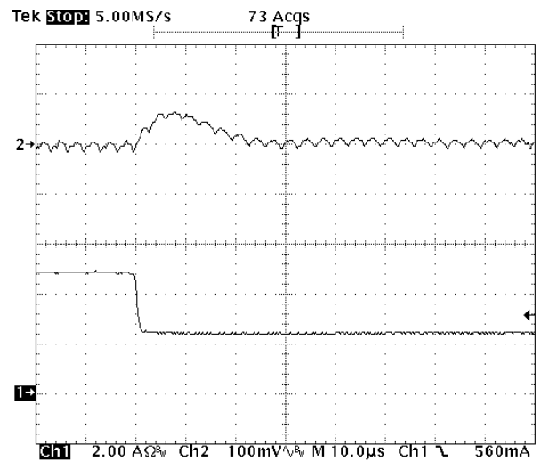
Fig-1.0V-7: Output voltage response for V_{out}=1.0V to positive load current step-change from 5A to 2.5A with slew rate of -5A/\mu s at V_{in}=5.0V . C_o=47\mu F \times 2 ceramic.
