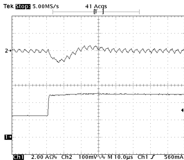
Fig-2.0V-6: Output voltage response for V_{out}=2.0V to positive load current step-change from 2.5A to 5A with slew rate of 5A/\mu s at V_{in}=5.0V . C_o=47\mu F \times 2 ceramic.
