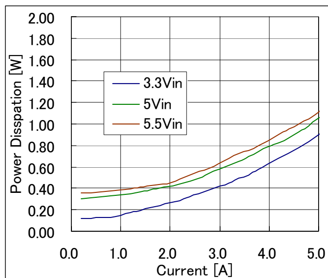
Fig-2.5V-3: Power dissipation vs. load current and input voltage for Vout=2.5V. Airflow rate=200 LFM (1.0m/s) and Ta=25°C.
