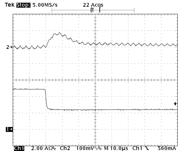
Fig-3.3V-7: Output voltage response for V_{out}=3.3V to negative load current step-change from 5A to 2.5A with slew rate of -5A/\mu s at V_{in}=5.0V . C_o=47\mu F \times 2 ceramic.
