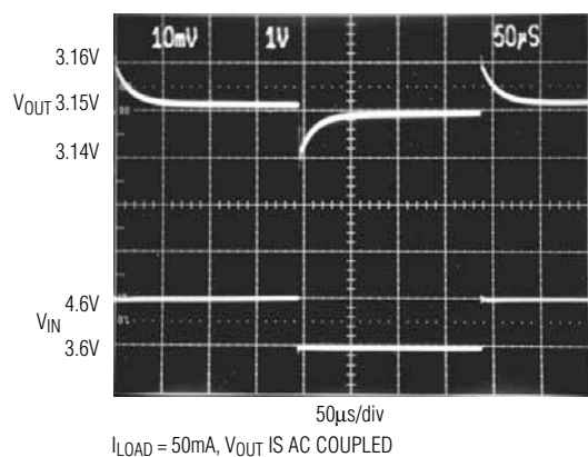
LINE TRANSIENT
