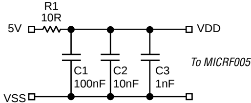
Figure 8. Supply Bypassing
