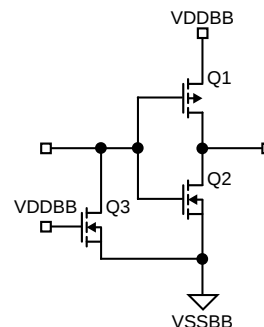
Figure 7. T/R Pin
