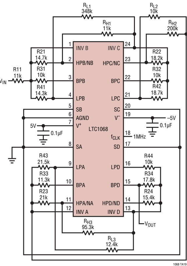
FilterCAD Custom Inputs for f_c = 10\text{kHz}
