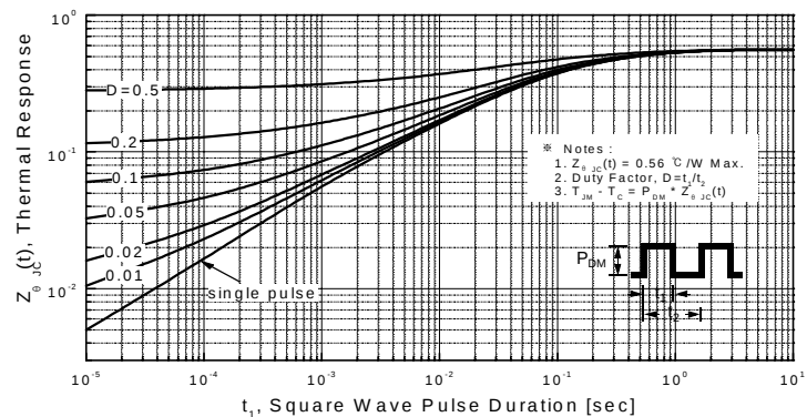
Figure 11-1. Transient Thermal Response Curve for FQP12N60C
