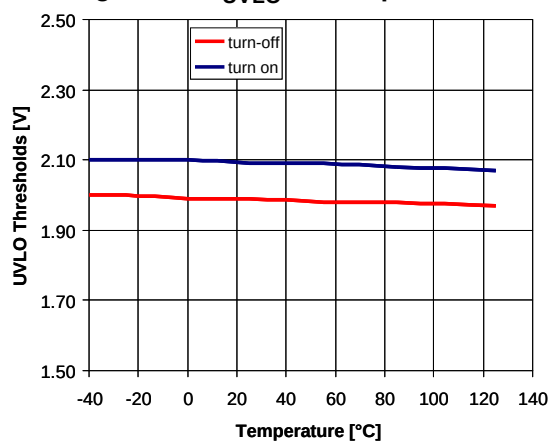
Figure 10. V_{UVLO} vs. temperature
