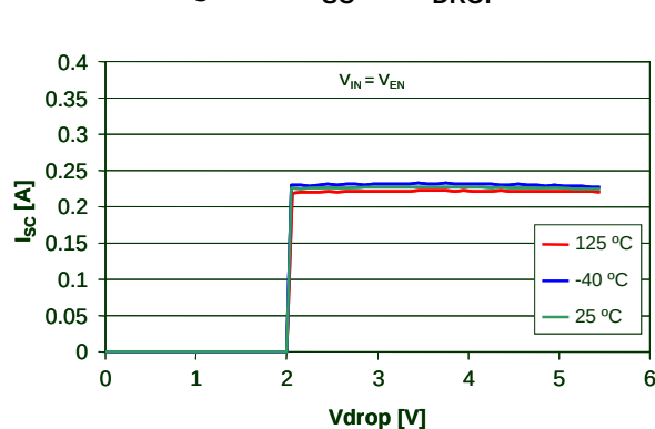
Figure 14. I_{SC} vs. V_{DROP}
