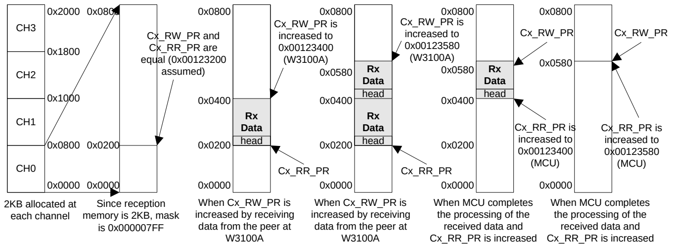
UDP Reception Memory Management for Each Channel
