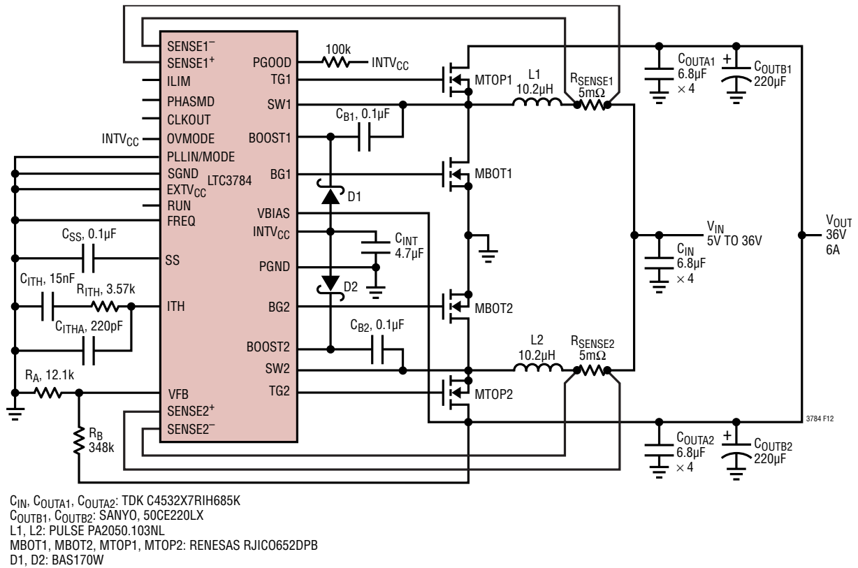
Figure 12. High Efficiency 2-Phase 36V Boost Converter
