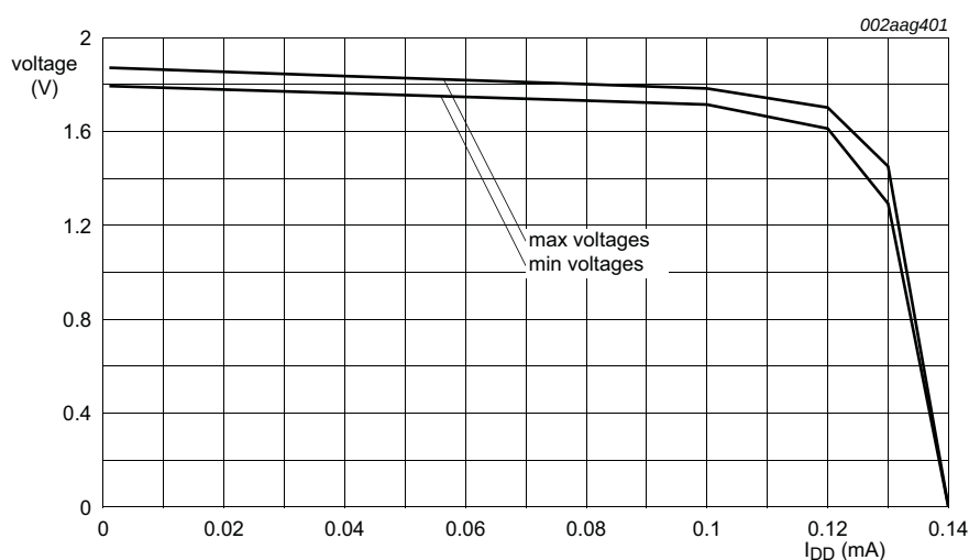
Fig 20. LDO3 PSU voltage drop (V) vs. current draw (mA), LDO3 @ 1.8 V
