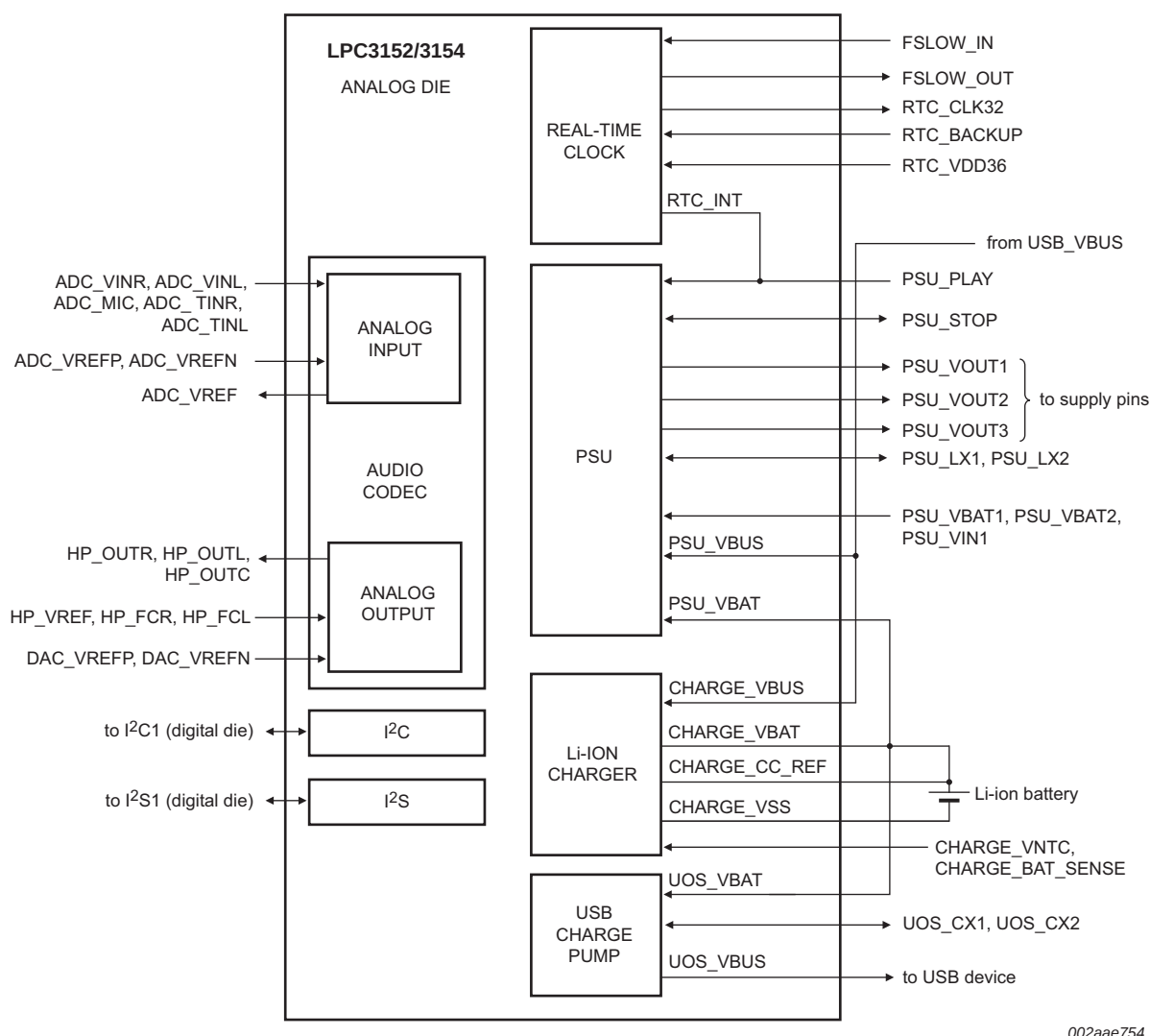
Fig 11. Block diagram of the analog die
