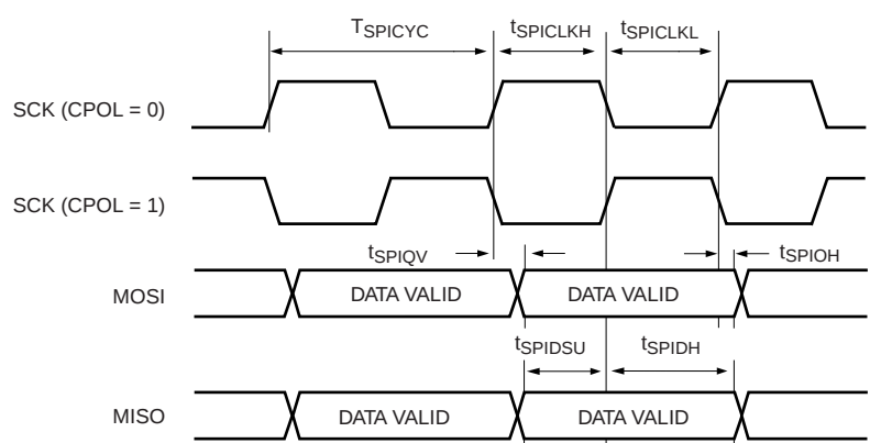
Fig 37. SPI master timing (CPHA = 1)
