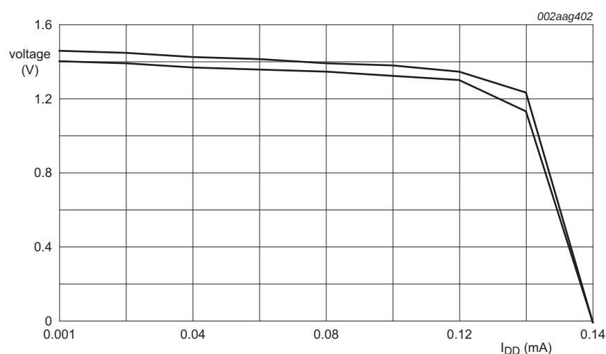
Fig 21. LDO3 PSU voltage drop (V) vs. current draw (mA), LDO3 @ 1.4 V
