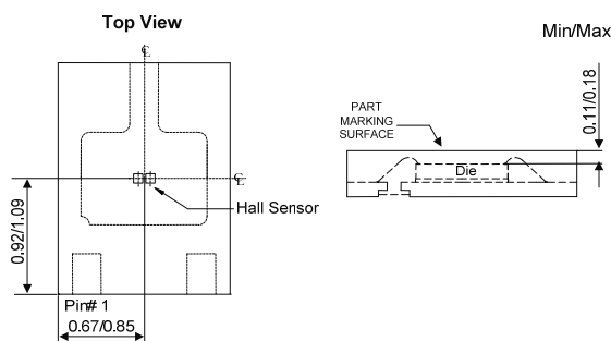
Sensor Location
