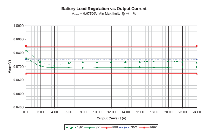
Figure 2 – Battery Mode Line and Load Regulation
