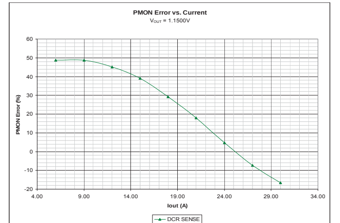
Figure 6 – Typical PMON Error v/s Output Current
