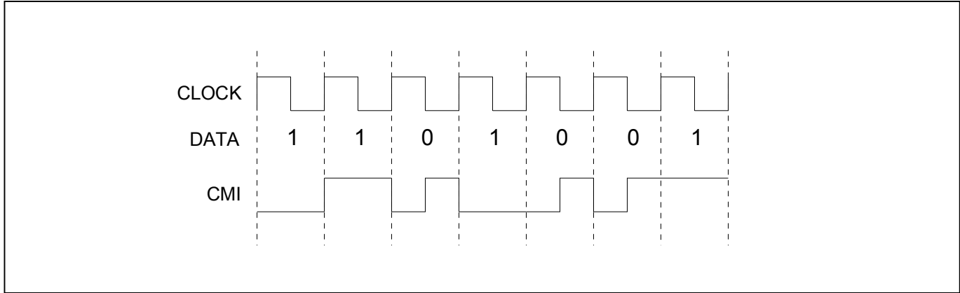
Figure 17-1. CMI Coding
