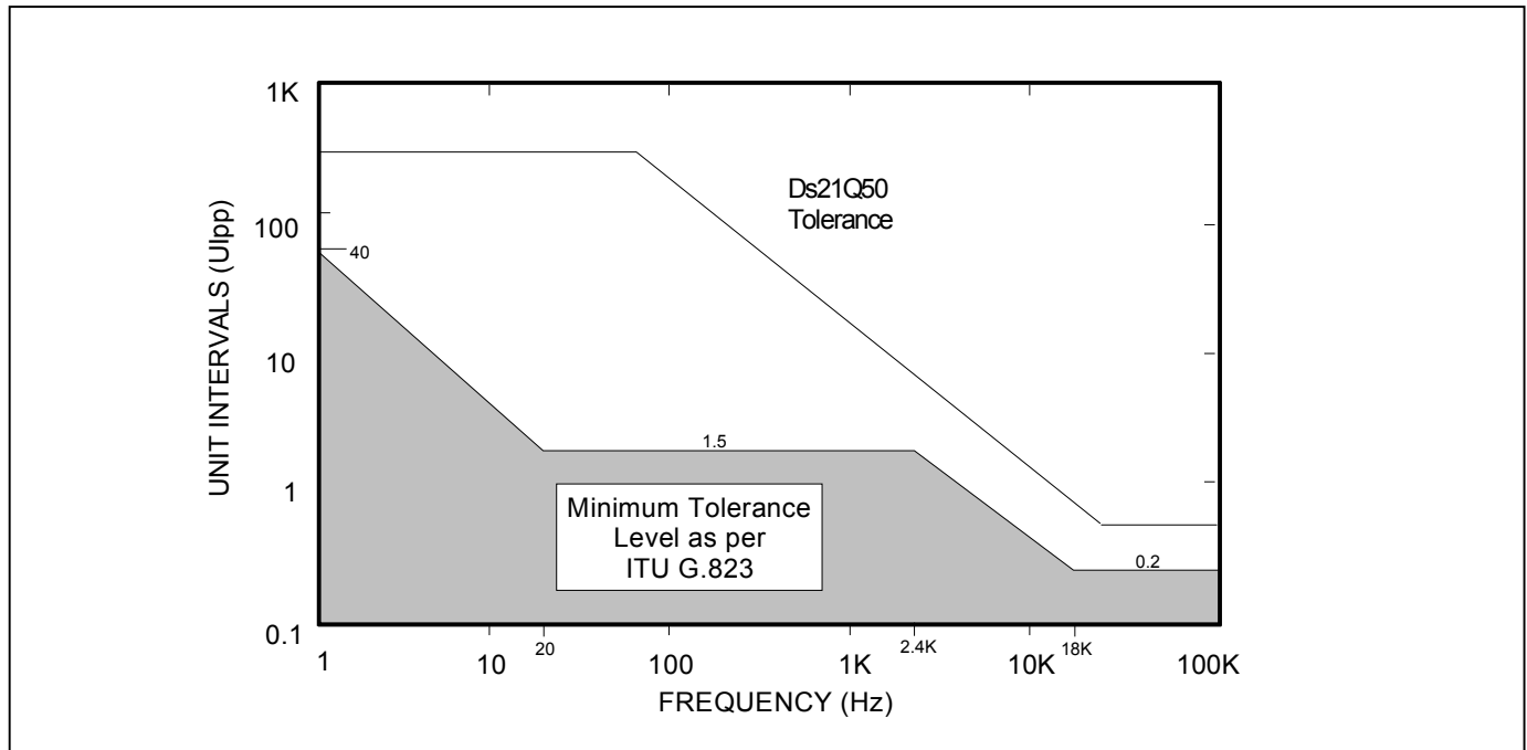
Figure 16-5. Jitter Tolerance
