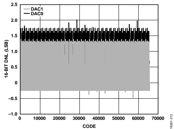
Figure 38. DNL, I_{OUTFS} = 15.6 mA, 16-Bit Resolution
