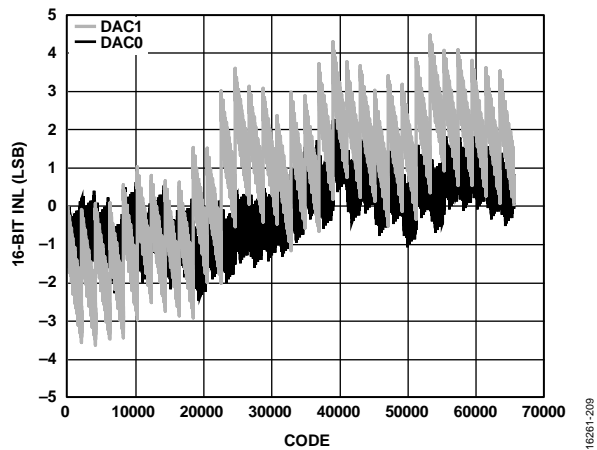
Figure 35. INL, I_{OUTFS} = 26 mA, 16-Bit Resolution
