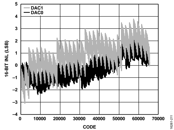
Figure 37. INL, I_{OUTFS} = 20 mA, 16-Bit Resolution
