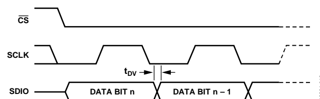
Figure 47. Timing Diagram for Serial Port Register Read
