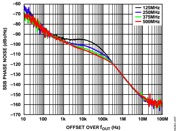
Figure 33. Single-Sideband (SSB) Phase Noise vs. Offset over f_{OUT} , over PFD Frequency, f_{DAC} = 12 GHz, f_{OUT} = 1.8 GHz, PLL On, PLL Reference Clock = 500 MHz
