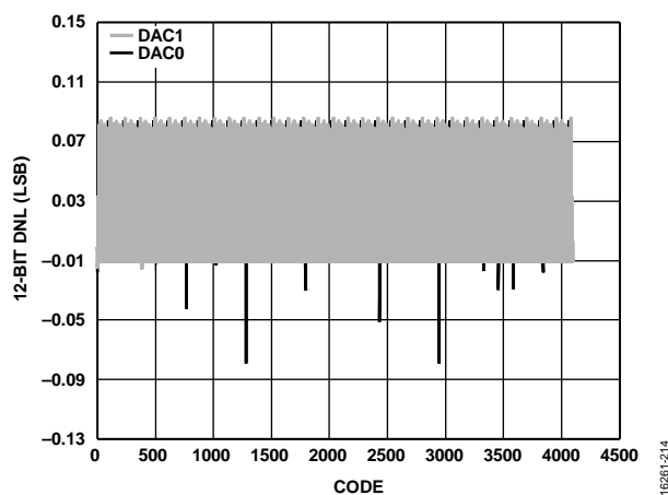
Figure 40. DNL, I_{OUTFS} = 20 mA, 12-Bit Resolution
