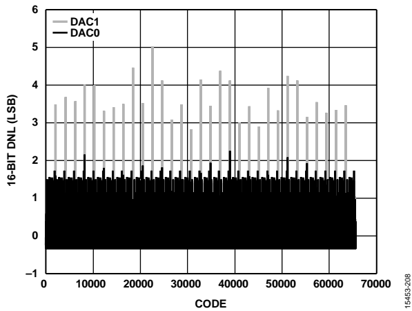
Figure 34. DNL, I_{OUTFS} = 26 mA, 16-Bit Resolution
