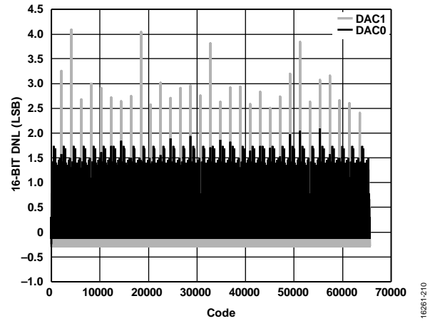
Figure 36. DNL, I_{OUTFS} = 20 mA, 16-Bit Resolution
