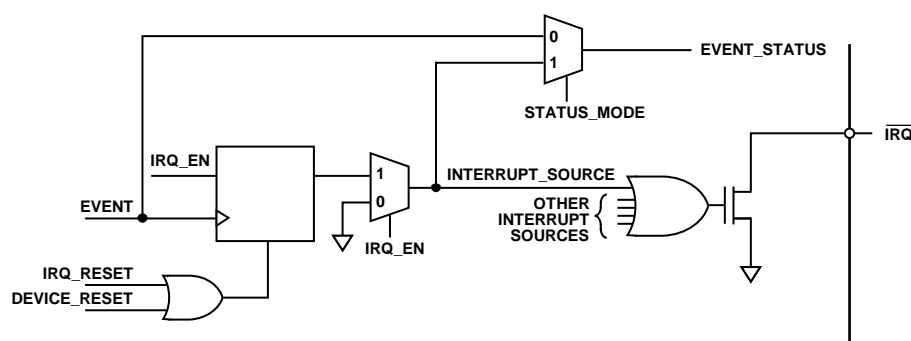
Figure 82. Simplified Schematic of \overline{IRQx} Circuitry
