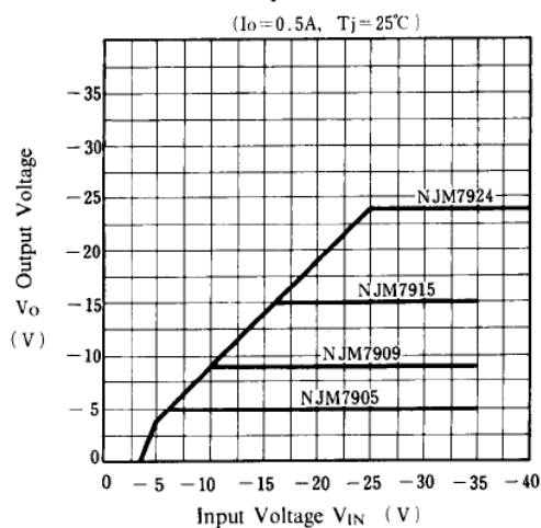
NJM7900 Output Characteristics
