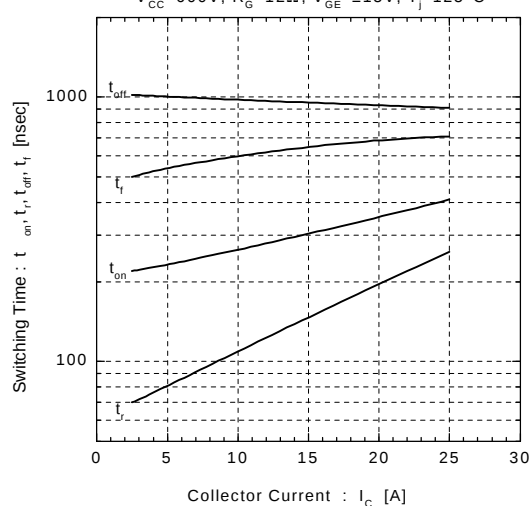
Switching Time vs. Collector Current V_{cc}=600V, R_G=12\Omega, V_{ge}=\pm 15V, T_J=125^\circ\text{C}
