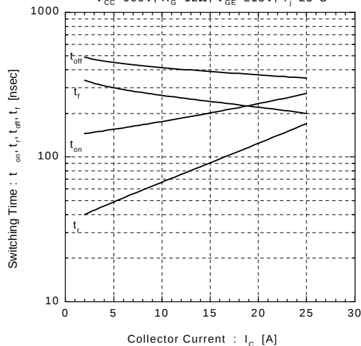
Switching Time vs. Collector Current V_{cc}=600V, R_G=12\Omega, V_{ge}=\pm 15V, T_J=25^\circ\text{C}
