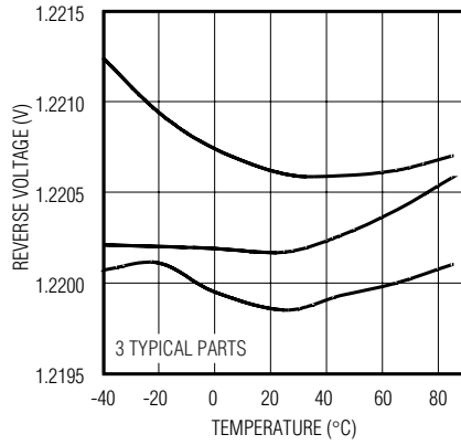
MAX6138_12 TEMPERATURE DRIFT
