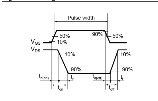
Fig.1-2 Switching Waveforms
