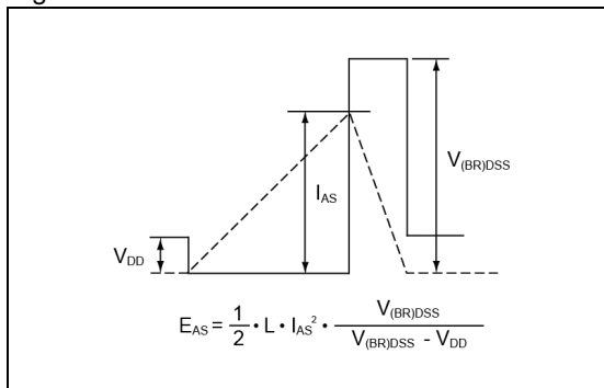
Fig.3-2 Avalanche Waveform
