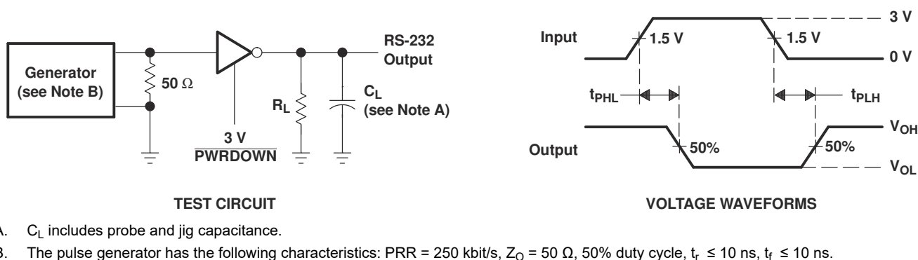
Figure 7-2. Driver Pulse Skew
