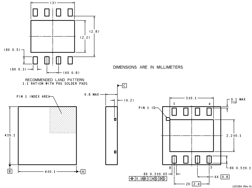
8-Lead LLP Order Number LM2940LD-5.0, LM2940LD-8.0, LM2940LD-9.0, LM2940LD-10, LM2940LD-12 or LM2940LD-15 NS Package Number LDC08A
