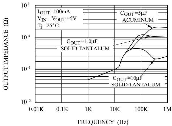
OUTPUT IMPEDANCE
