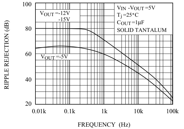
RIPPLE REJECTION
