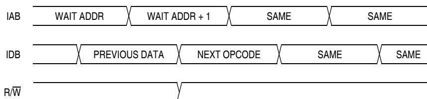
Figure 17-12. Wait Mode Entry Timing
