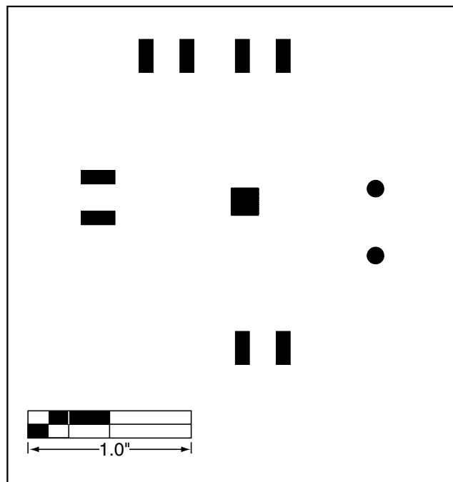
Figure 9. MAX9987/MAX9988 EV Kit PC Board Layout—Bottom Soldermask
