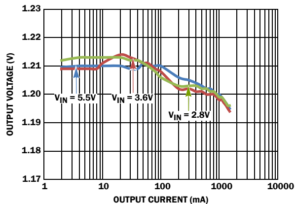
FIGURE 16. DCD OUTPUT VOLTAGE vs OUTPUT CURRENT ( V_{OUT} = 1.2V , PFM/PWM)
