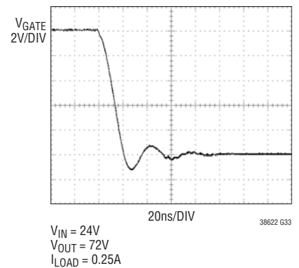
Gate Turn-Off Waveform Driving Renesas HAT2267H
