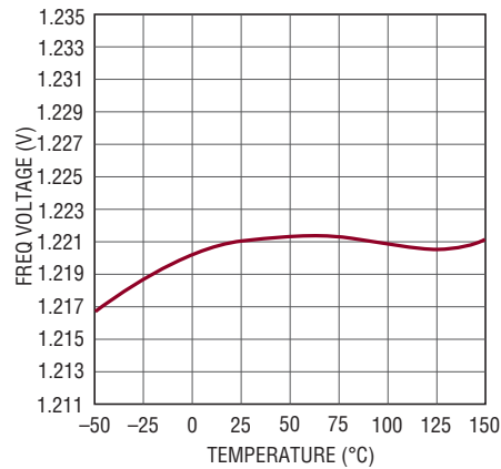
Frequency Pin Voltage vs Temperature
