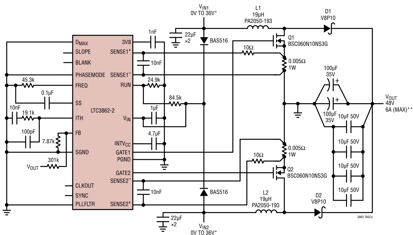
A 24V Dual Input, 48V/6A Output 2-Phase Boost Converter Application Circuit
