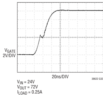
Gate Turn-On Waveform Driving Renesas HAT2267H
