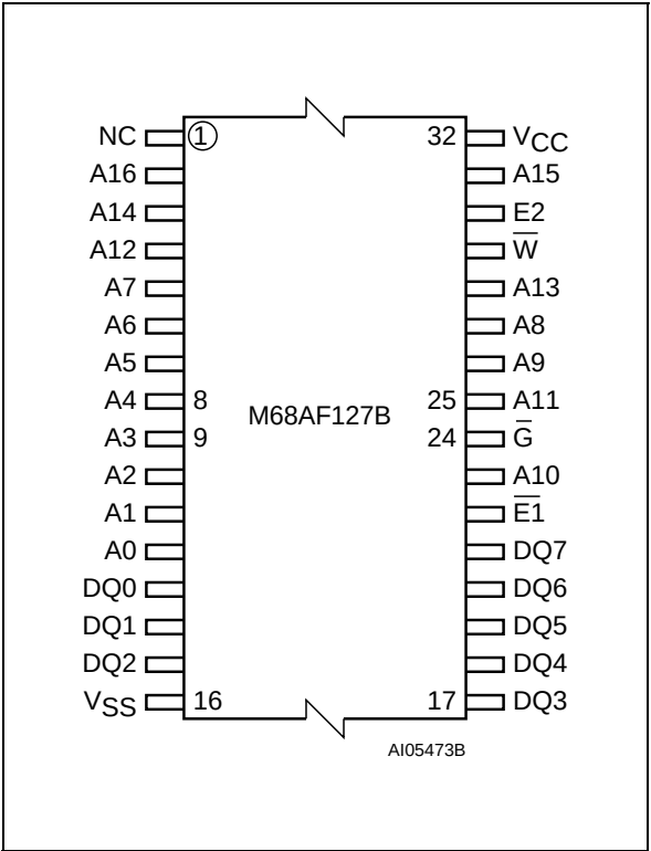
Figure 5. TSOP Connections
