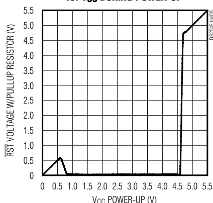
RST VOLTAGE vs. VCC DURING POWER-UP
