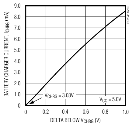
BATTERY CHARGER CURRENT vs. BATTERY VOLTAGE
