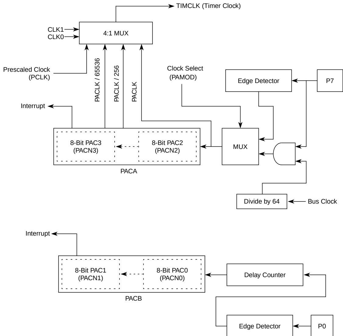
Figure 7-70. 16-Bit Pulse Accumulators Block Diagram
