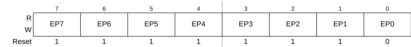
Figure 17-13. EEPROM Page Index Register (EPAGE)
