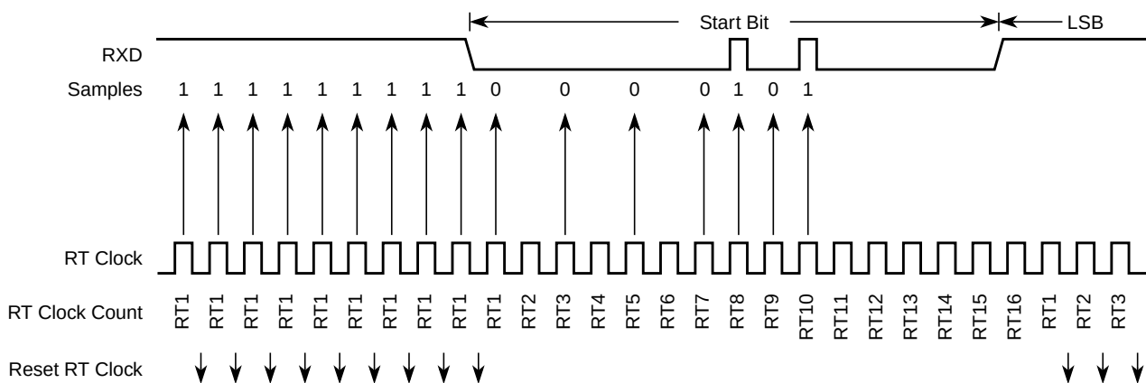
In Figure 11-27, a noise burst makes the majority of data samples RT8, RT9, and RT10 high. This sets the noise flag but does not reset the RT clock. In start bits only, the RT8, RT9, and RT10 data samples are ignored.
