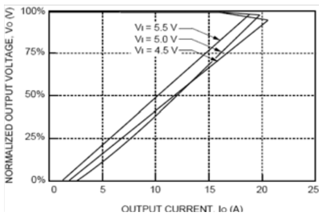
Figure 2. Typical Output Characteristics.
