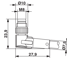
Dimensioned drawing
