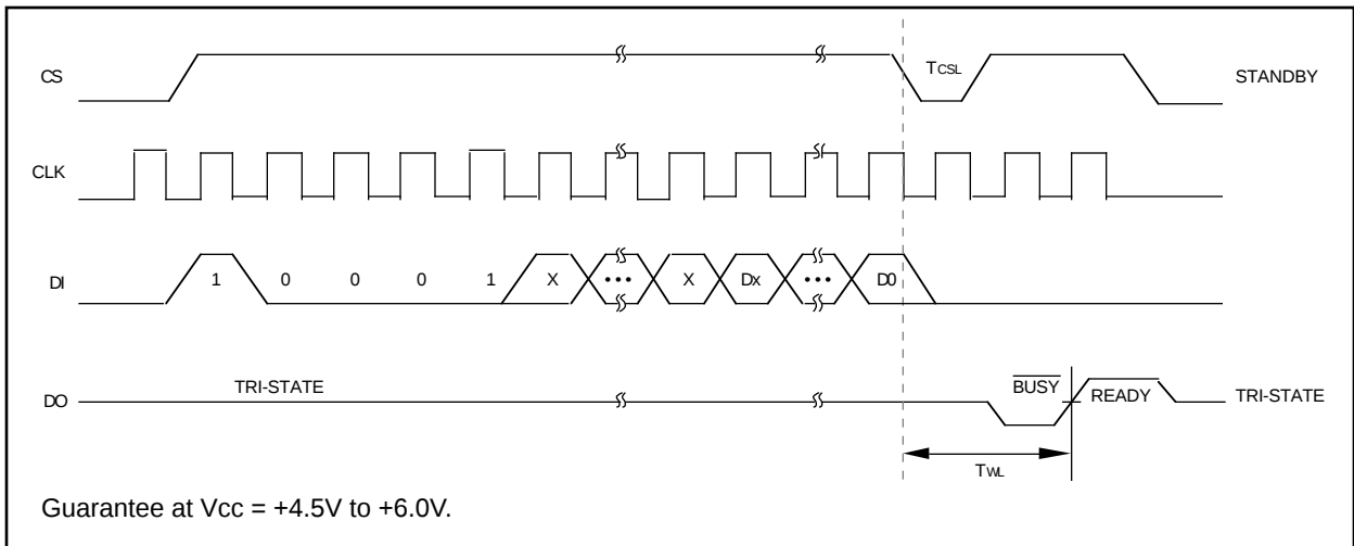
FIGURE 9-6: WRAL TIMING
