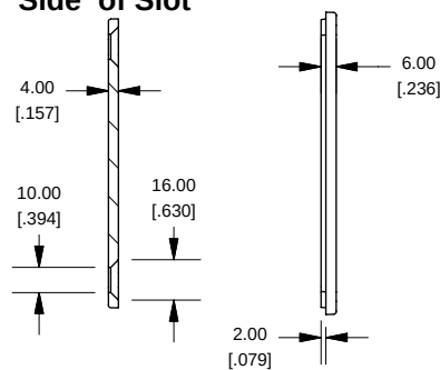
SECTION C-C Side of Slot
