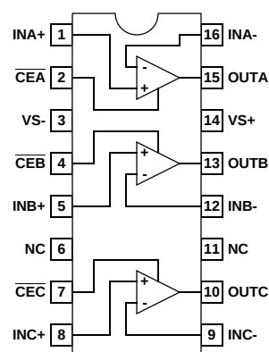
EL5392 [16 LD SOIC (0.150") & QSOP] TOP VIEW
