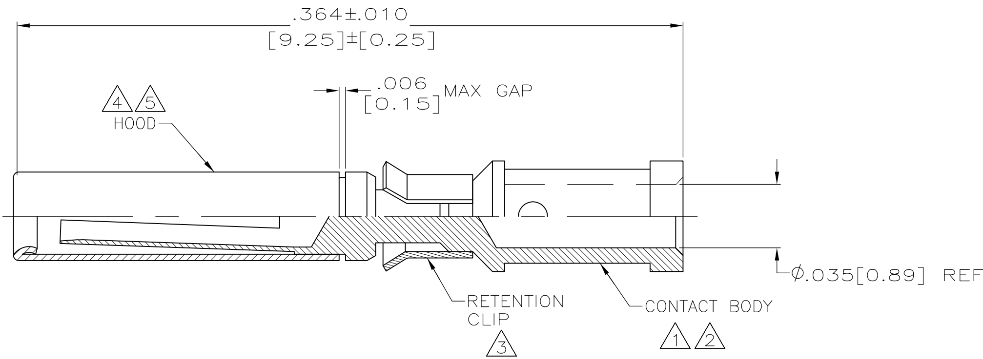
CONTACT ASSEMBLY
