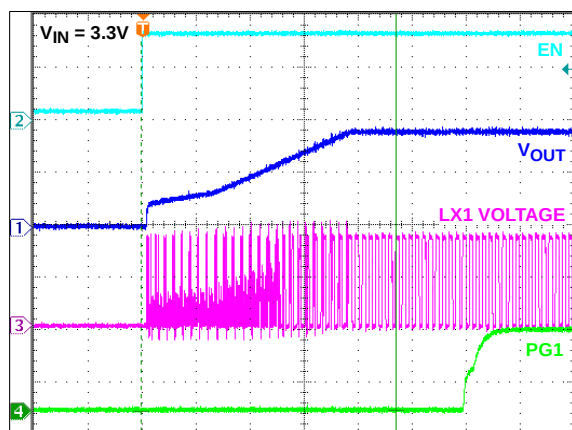
FIGURE 45. SOFT-START AT NO LOAD
