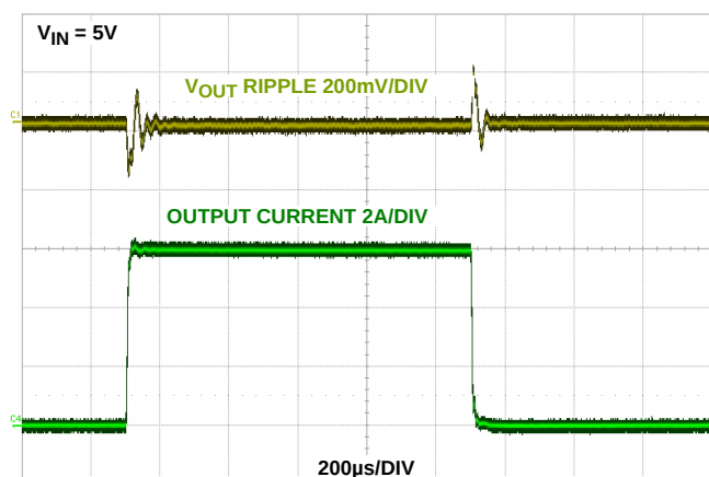
FIGURE 43. LOAD TRANSIENT RESPONSE
