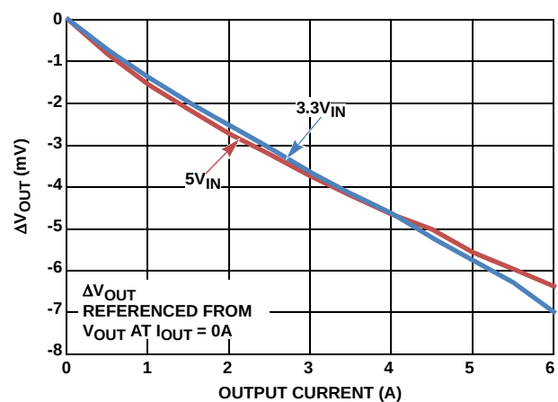
FIGURE 40. LOAD REGULATION, V_{OUT} = 1.8\text{V} , T_A = +25^\circ\text{C}
