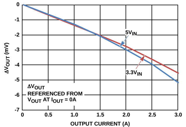
FIGURE 10. LOAD REGULATION, V_{OUT} = 1.8\text{V} , T_A = +25^\circ\text{C}
