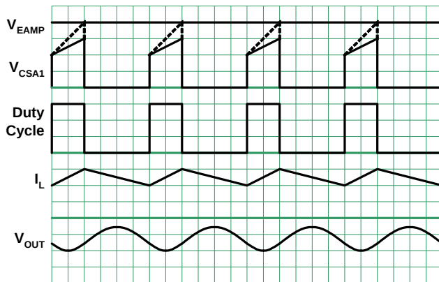
FIGURE 49. PWM OPERATION WAVEFORMS
