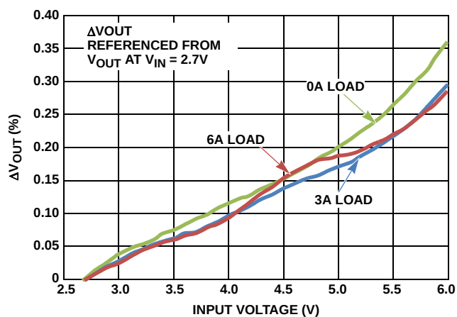
FIGURE 39. LINE REGULATION, V_{OUT} = 1.8\text{V} , T_A = +25^\circ\text{C}
