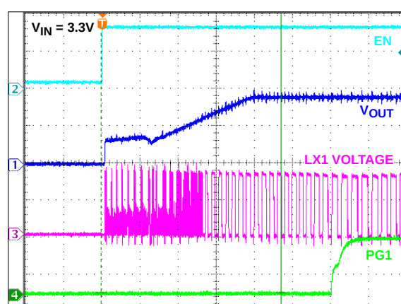
FIGURE 46. SOFT-START AT 6A LOAD
