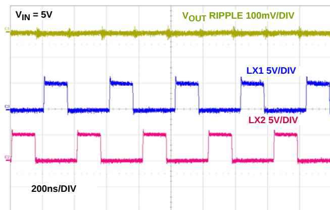
FIGURE 41. STEADY STATE OPERATION AT NO LOAD
