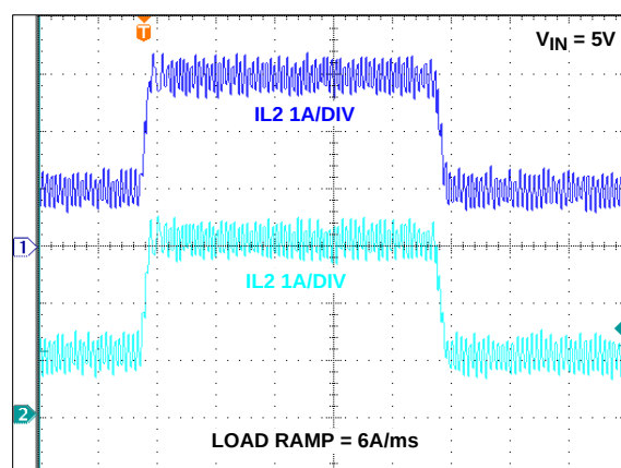
FIGURE 48. CURRENT SHARE BALANCING, 2A TO 6A
