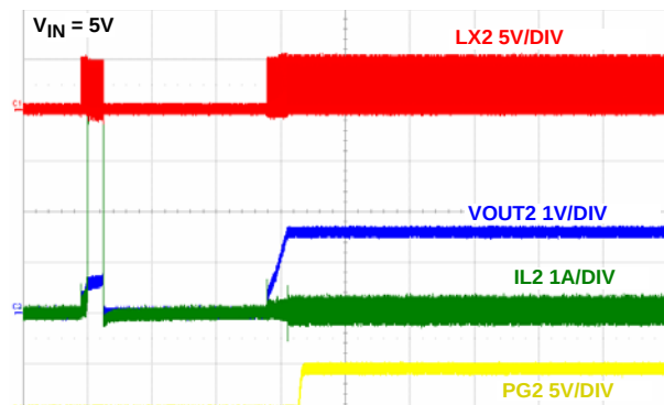
FIGURE 30. OUTPUT SHORT CIRCUIT RECOVERY (FROM HICUP) CHANNEL 2
