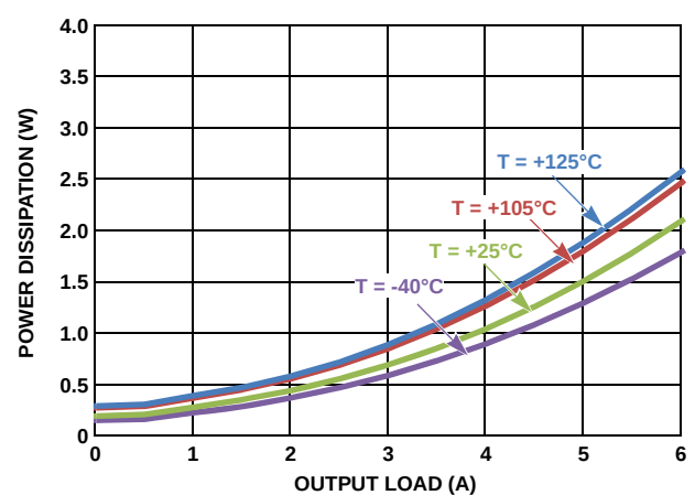
FIGURE 38. POWER DISSIPATION, V_{IN} = 5\text{V} , V_{OUT} = 1.8\text{V}
