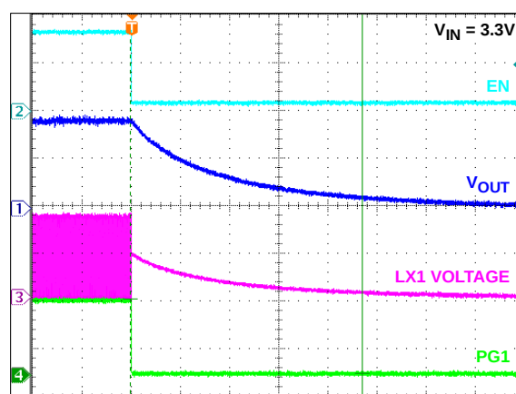
FIGURE 44. SOFT-DISCHARGE SHUTDOWN
