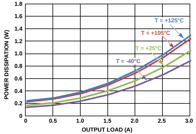
FIGURE 8. POWER DISSIPATION, V_{IN} = 5\text{V} , V_{OUT} = 1.8\text{V}
