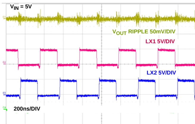
FIGURE 42. STEADY STATE OPERATION AT 6A LOAD
