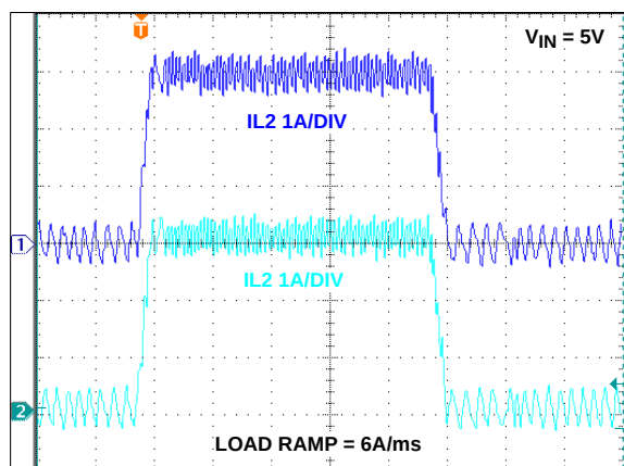
FIGURE 47. CURRENT SHARE BALANCING, 0A TO 6A
