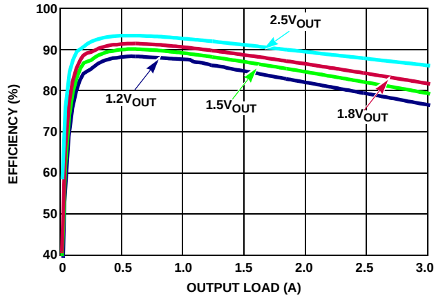
FIGURE 5. EFFICIENCY, V_{IN} = 3.3\text{V} , T_A = +25^\circ\text{C}
