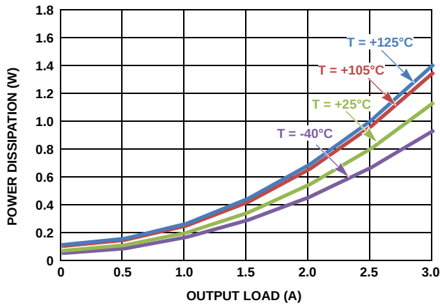
FIGURE 7. POWER DISSIPATION, V_{IN} = 3.3\text{V} , V_{OUT} = 1.8\text{V}
