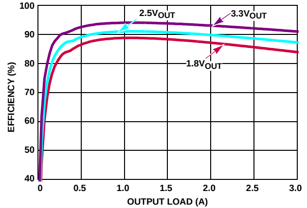
FIGURE 6. EFFICIENCY, V_{IN} = 5\text{V} , T_A = +25^\circ\text{C}
