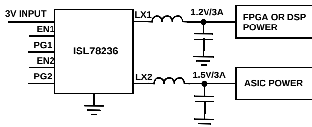
FIGURE 1. TYPICAL APPLICATION BLOCK DIAGRAM: DUAL OUTPUT 3A/3A BUCK REGULATOR
