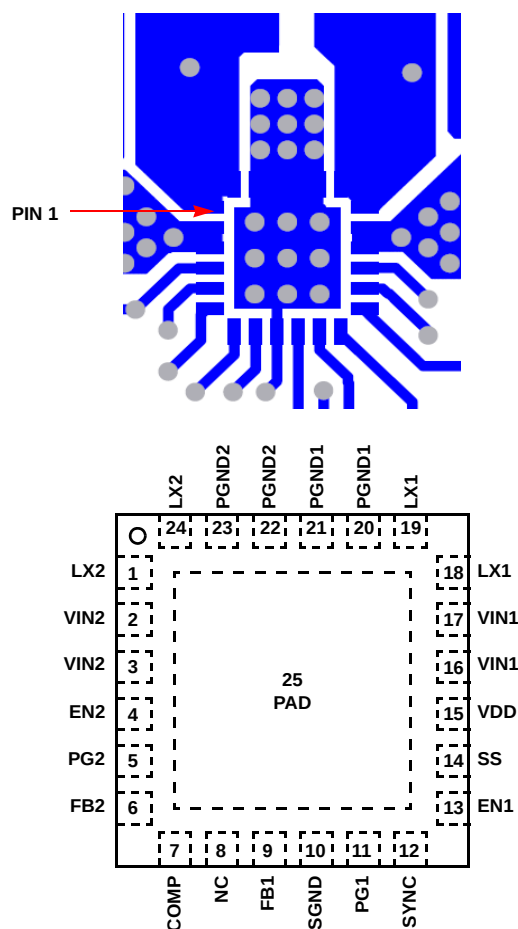
FIGURE 52. RECOMMENDED THERMAL PAD LAYOUT
