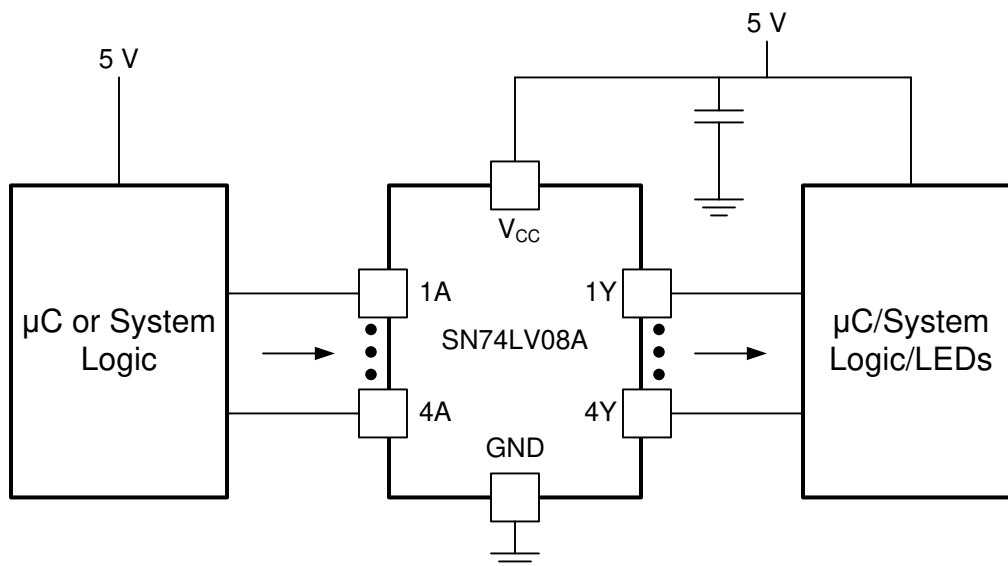
Figure 8-1. Application Diagram
