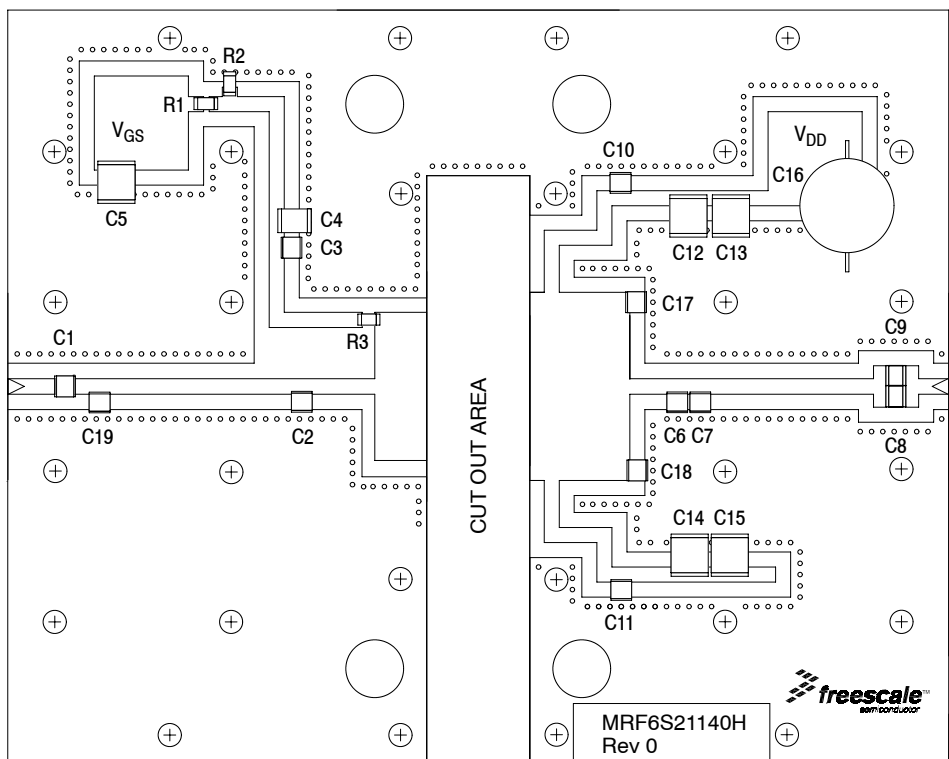
Figure 2. MRF6S21140HR3(HSR3) Test Circuit Component Layout
