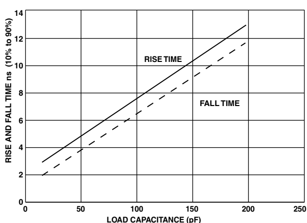
Figure 49. Typical Rise and Fall Times (10% to 90%) vs. Load Capacitance for Driver D at V_{DDEXT} (max)
