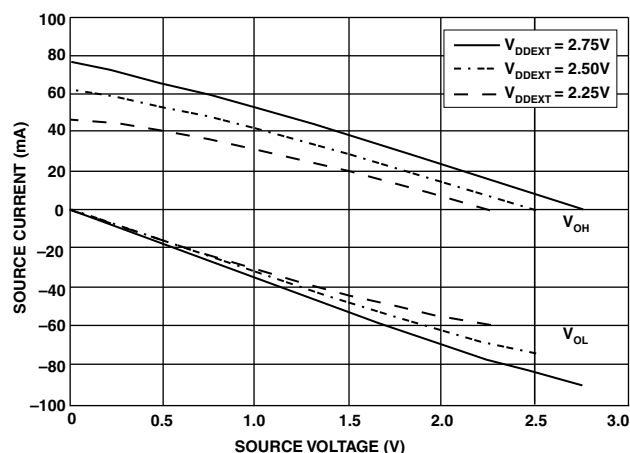
Figure 37. Drive Current D (Low V_{DDEXT} )
