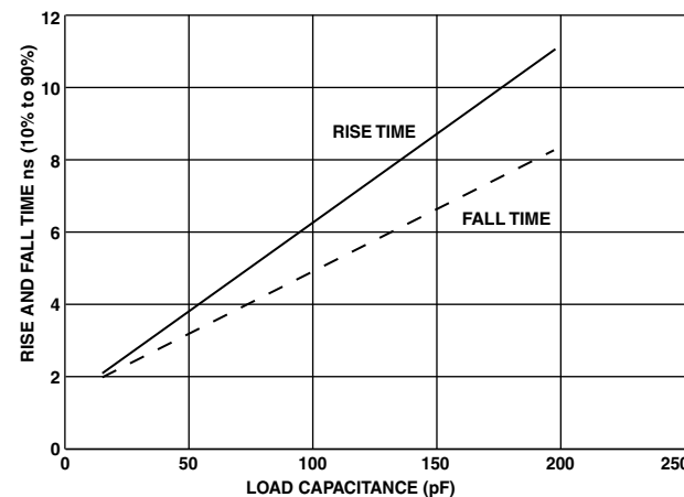
Figure 44. Typical Rise and Fall Times (10% to 90%) vs. Load Capacitance for Driver B at V_{DDEXT} (min)
