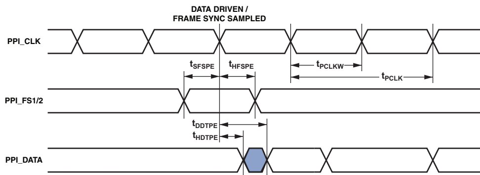
Figure 17. PPI GP Tx Mode with External Frame Sync Timing (PLL_CTL Bit 4 = 1)
