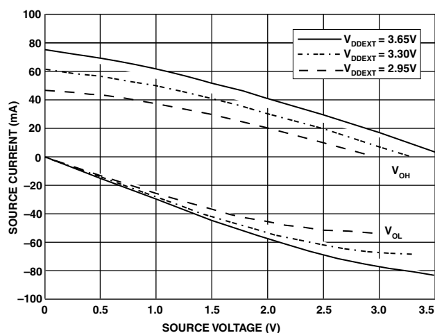
Figure 36. Drive Current C (High V_{DDEXT} )
