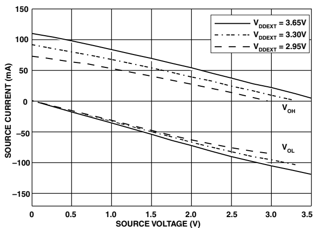
Figure 38. Drive Current D (High V_{DDEXT} )
