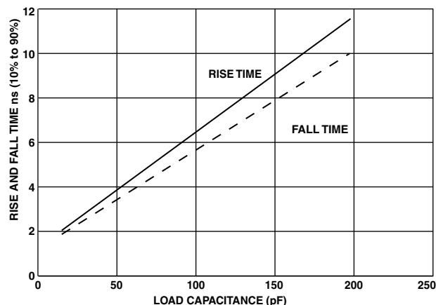
Figure 43. Typical Rise and Fall Times (10% to 90%) vs. Load Capacitance for Driver A at V_{DDEXT}(\text{max})
