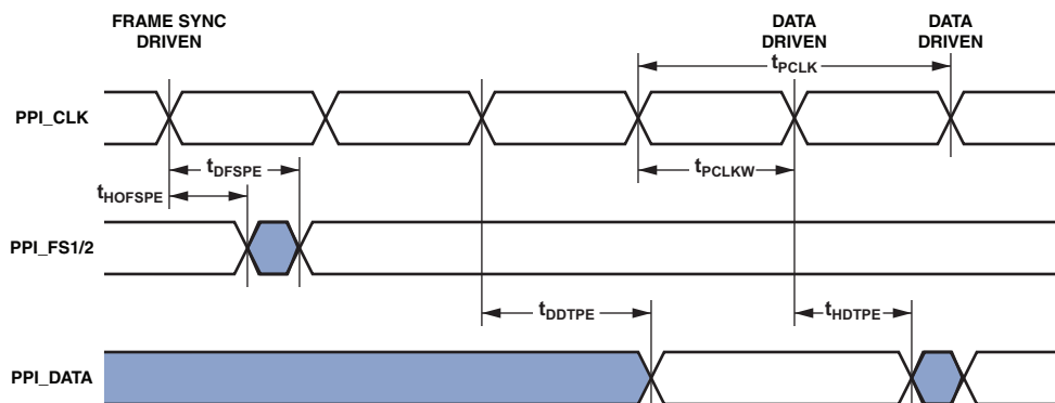
Figure 16. PPI GP Tx Mode with Internal Frame Sync Timing
