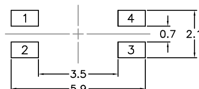
RECOMMENDED FOOTPRINT
