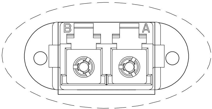
DETAIL C TYP. 6 PLC.
