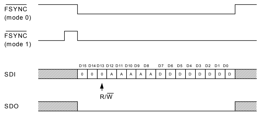
Figure 16. Secondary Communication Data Format—Write Cycle
