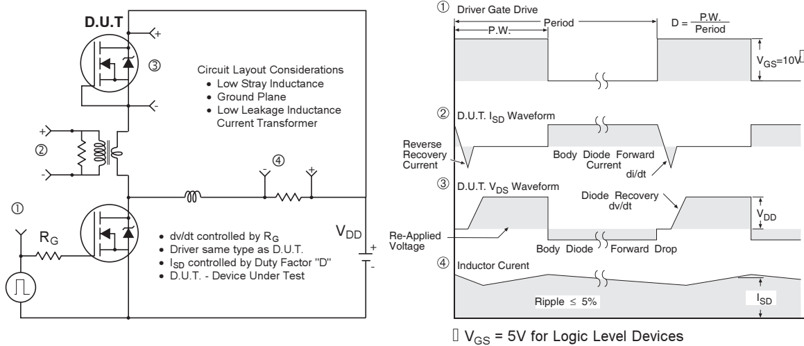
Fig 15. for N-Channel HEXFET ® Power MOSFETs
