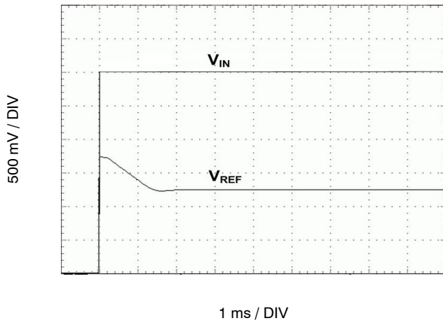
Figure 14. Turn-On Time
