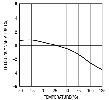
Frequency Variation vs Temperature
