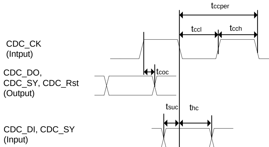
Figure 11. CODEC Timing
