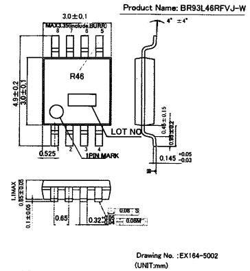
Fig4-(f) PHYSICAL DIMENSION TSSOP-B8J (BR93L46RFVJ-W)
