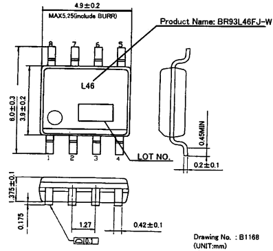
Fig4-(d) PHYSICAL DIMENSION SOP-J8 (BR93L46FJ-W)
