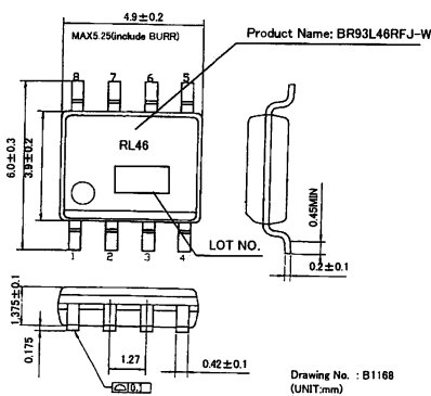
Fig4-(e) PHYSICAL DIMENSION SOP-J8 (BR93L46RFJ-W)
