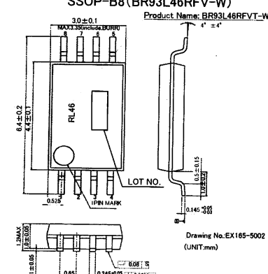
Fig4-(j) PHYSICAL DIMENSION TSSOP-B8 (BR93L46RFVT-W)
