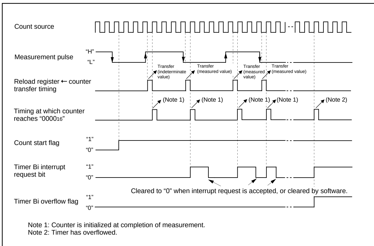
Figure 1.15.21. Operation timing when measuring a pulse width
