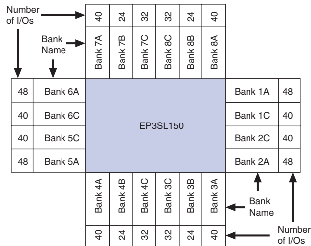
Figure 2-3. EP3SL150F1152 Device I/O Bank Resources
