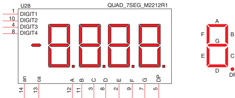
Figure 2-9. 7-Segment Display
