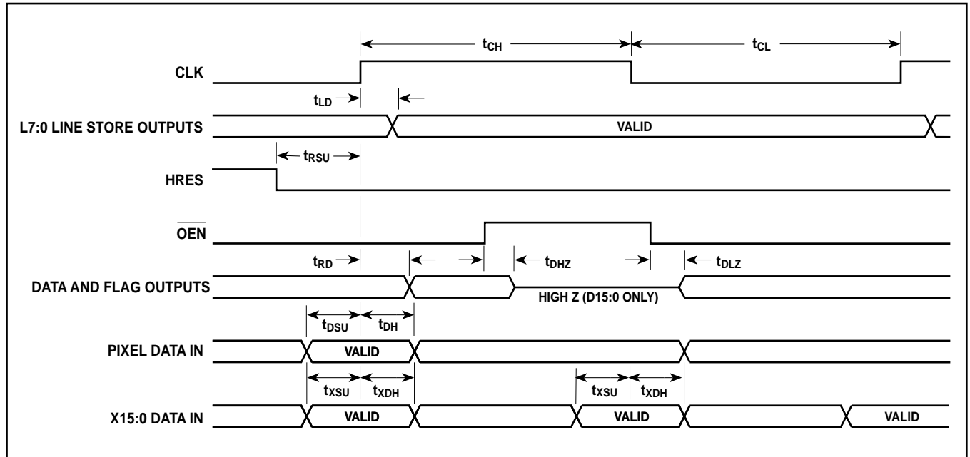
Fig. 12 Operational timing
