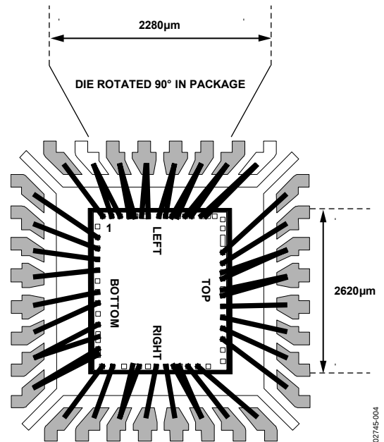
Figure 6. Bonding Diagram
